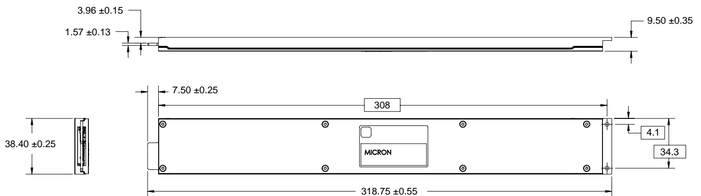
Figure 3: E1.L 9.5mm Nominal Dimensions
